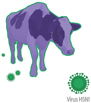
Virus H5N1
